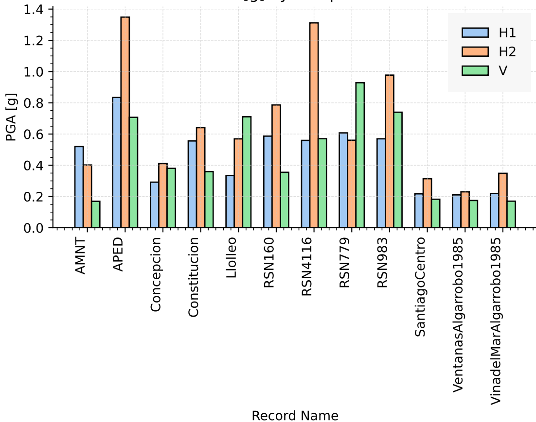
PGA [g] by Component
